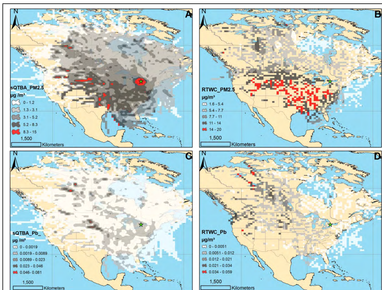
Figure 4. Comparisons of source regions identified by sQTBA (A–C) and RTWC (B–D) for PM 2.5 and Pb monitored at the OMOE Etobicoke South research station for the entire one year period (December 01, 2010–November 30, 2011).
