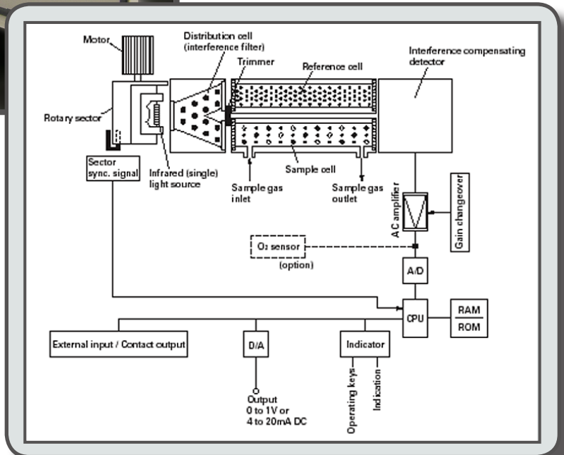
Principle diagram of NDIR type measurement (for NO, CO 2 , CO, CH 4 , SO 2 )
