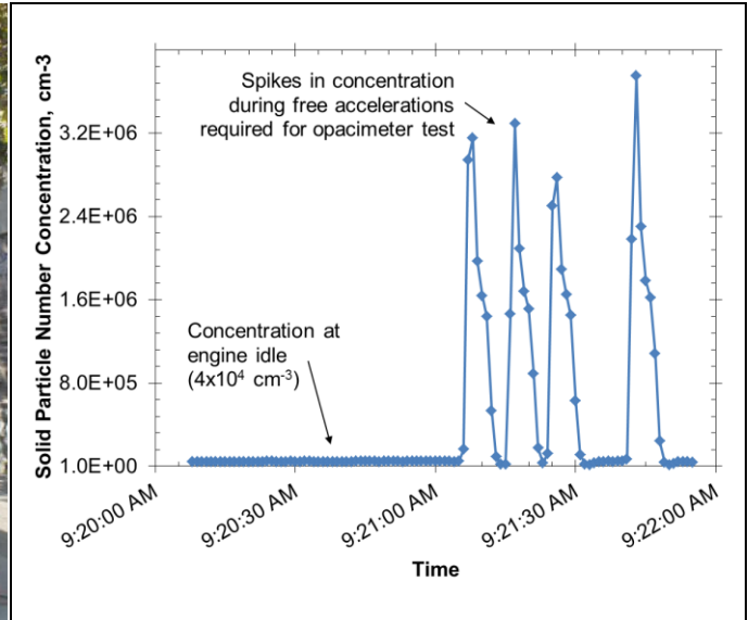
Figure 5: Measurements of solid particle numbers emitted by bus BIFY4 at idle and during free accelerations
